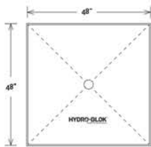
4' x 4' Shower Pan
