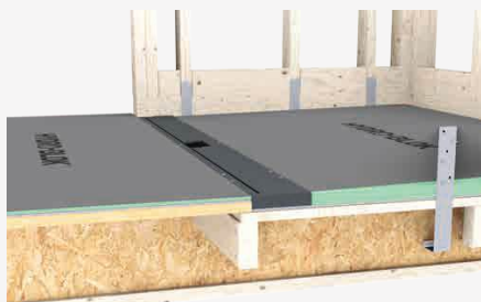
Single Slope Shower Pans
