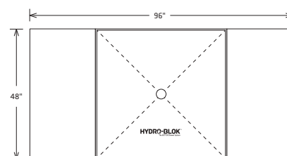
4' x 4' Shower Pan with two 4' x 2' Pan Extensions
