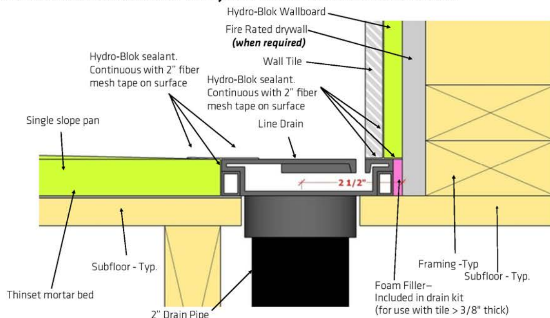
LINE DRAIN TO WALLBOARD & PAN JOINT DETAIL AT FIRE RATED WALL
