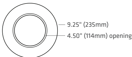
4 1/2" Mixer Valve Seal (9 1/4" dia.) SKU: HBVALVESEAL
