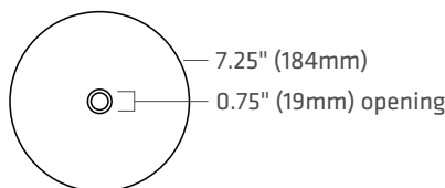
3/4" Pipe Seal (7 1/4" dia.) SKU: HBPIPESEAL
